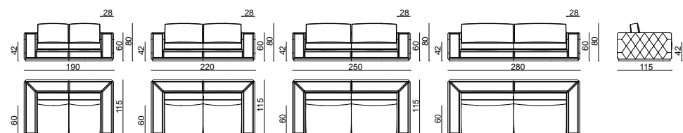
DIVANO / SOFA
